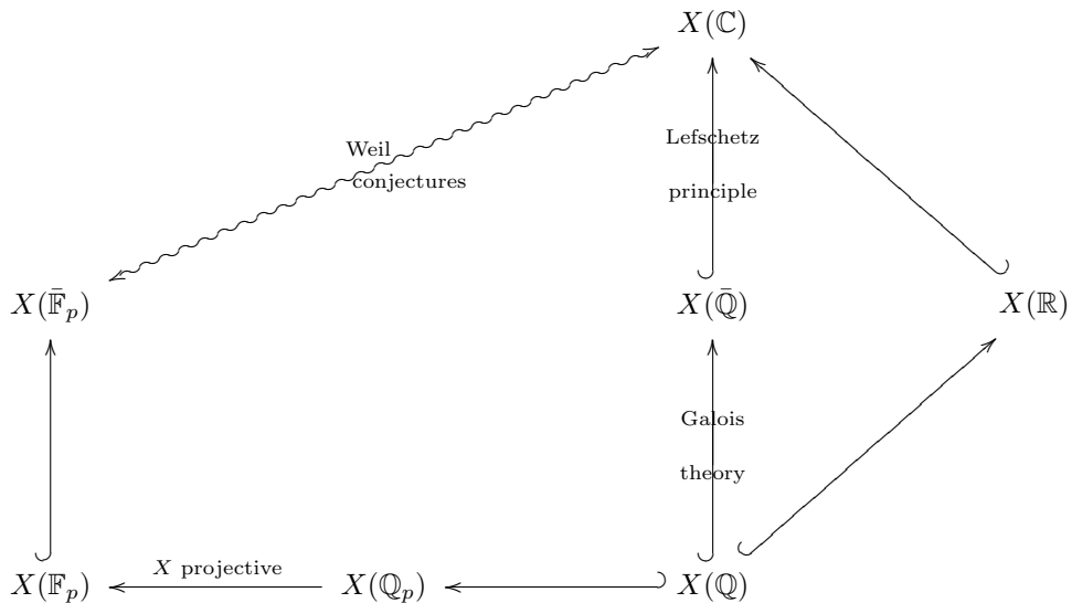
Figure 1: Some of the sets of points associated to a Diophantine equation
